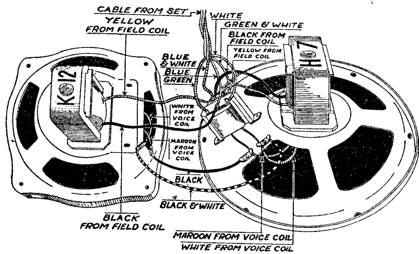
Speaker Connections
